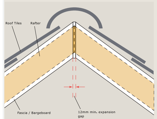
Fig. 22 Bargeboard at gable end showing apex.
