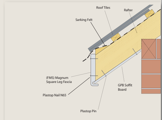
Fig 20c. Inclined soffit application with GPB soffit.
